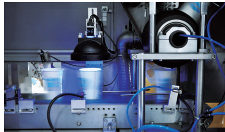
Inspection Machine
